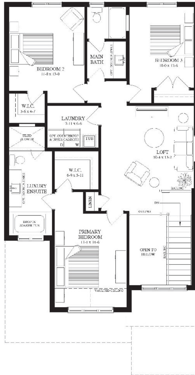
SECOND FLOOR 1244 Sq. Ft.
