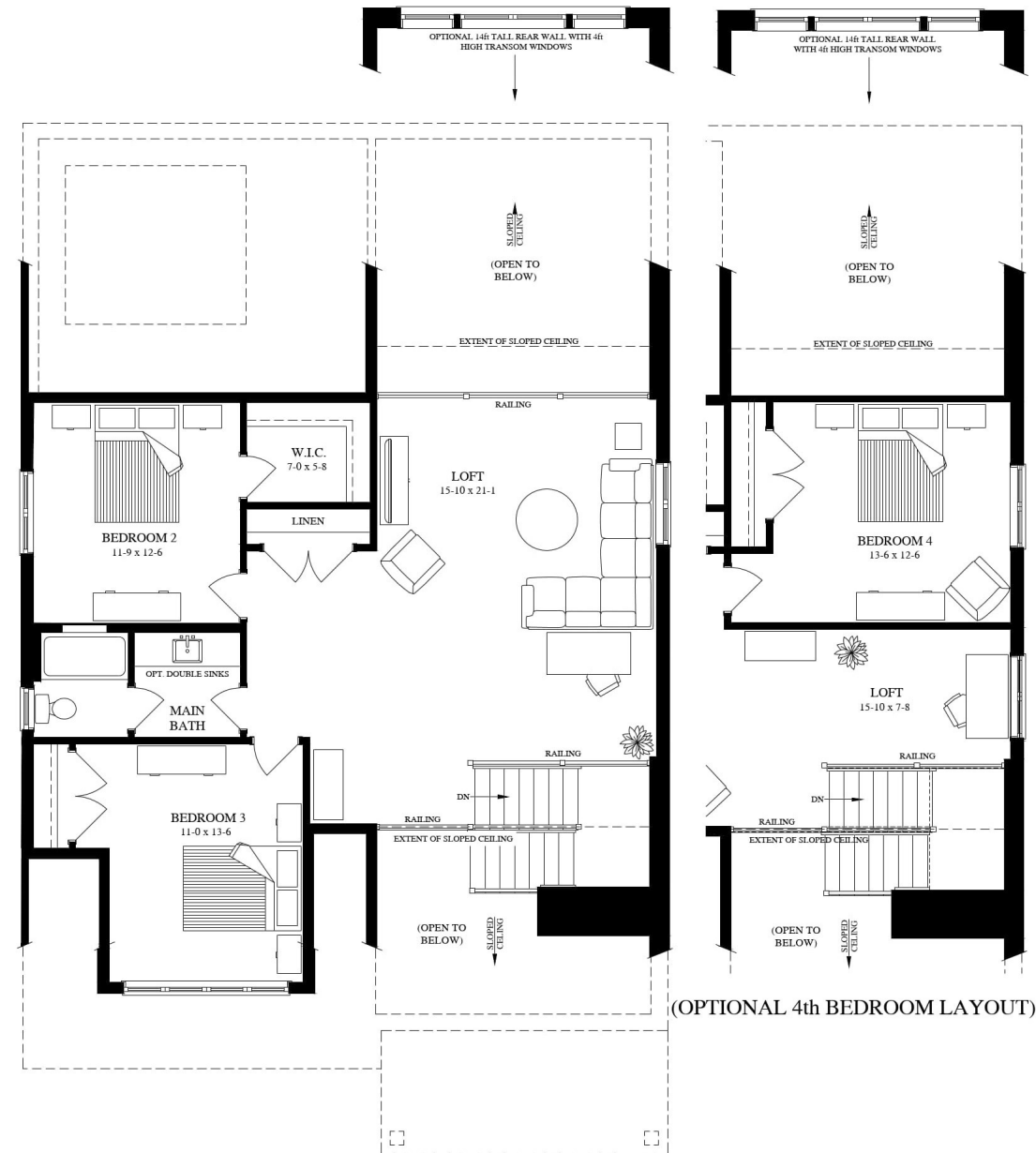
SECOND FLOOR 1063 Sq. Ft.
