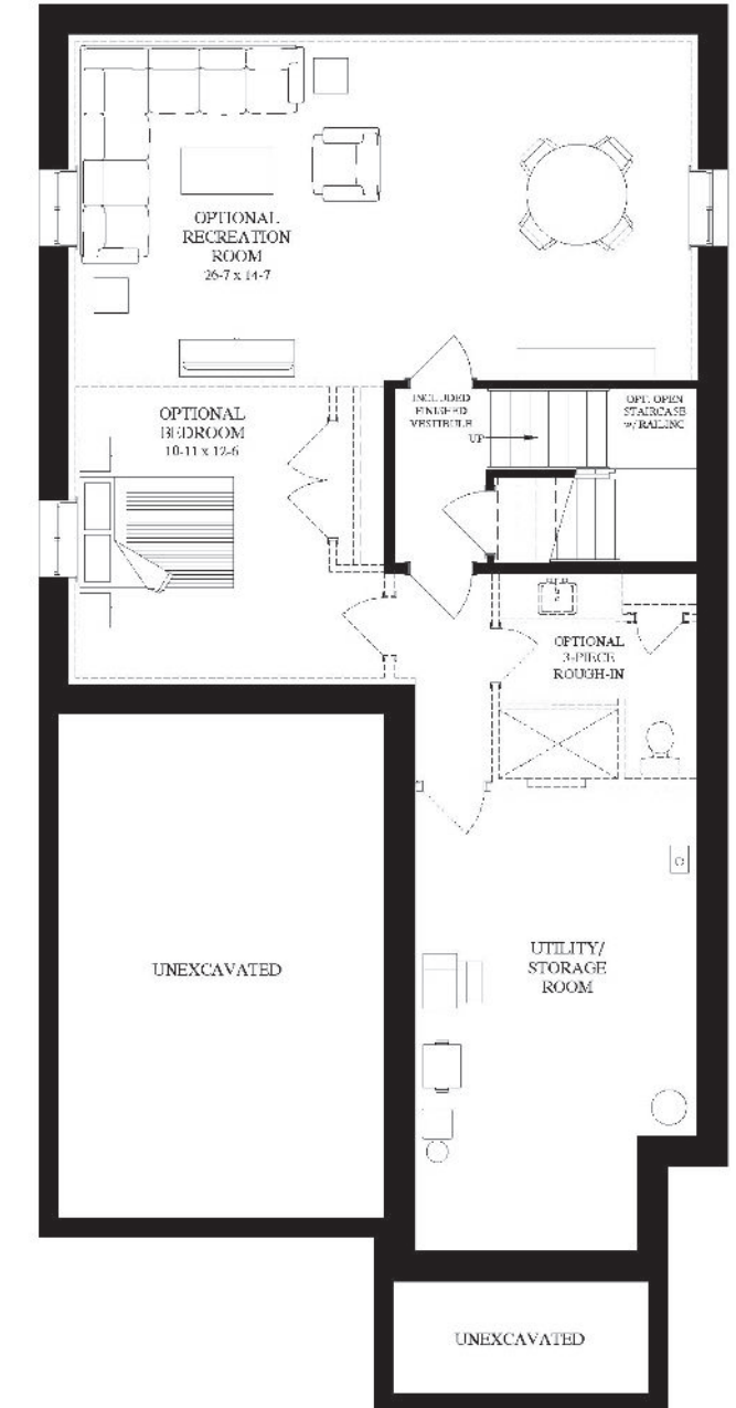
BASEMENT 966 Sq. Ft. Optional Finished Basement * Includes 125 Sq. Ft. finished vestibule
