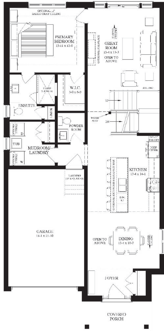
MAIN FLOOR 1274 Sq. Ft.
