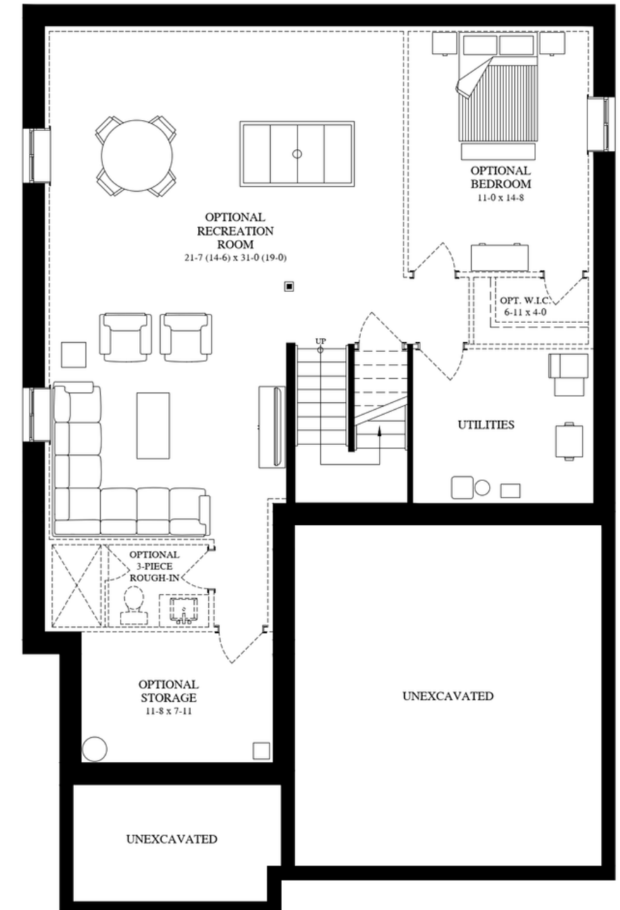
BASEMENT 1268 Sq. Ft. Optional Finished Basement
