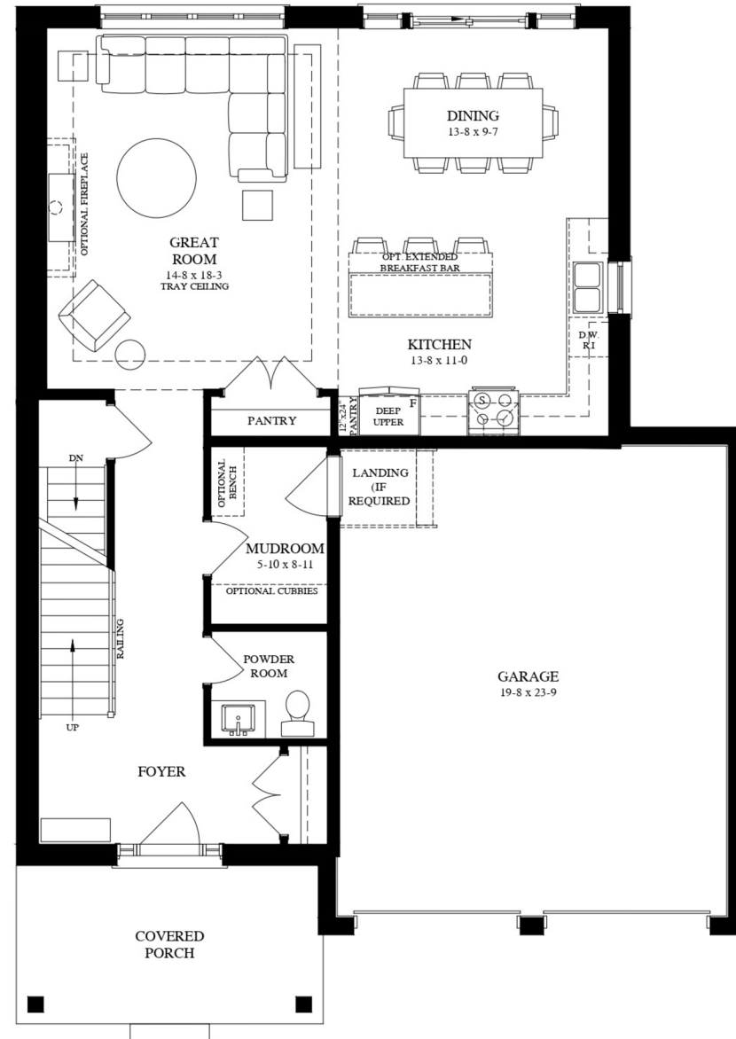
MAIN FLOOR 1021 Sq. Ft.
