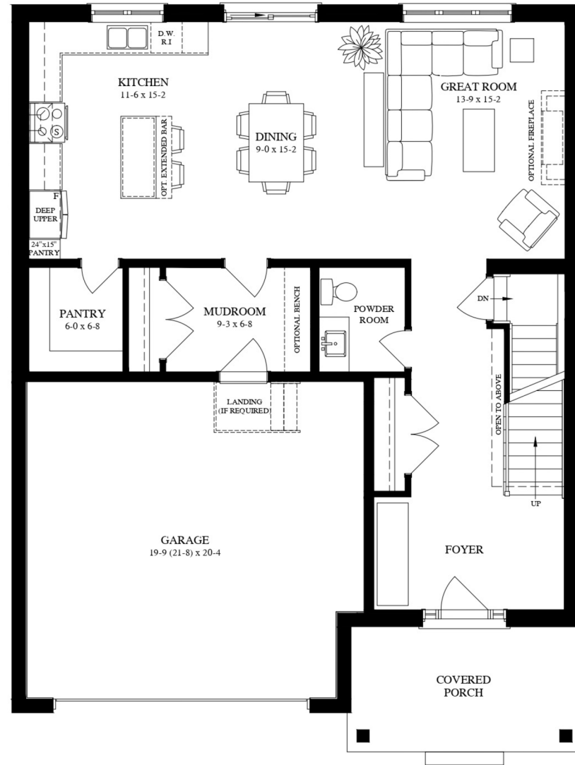
MAIN FLOOR 1079 Sq. Ft.
