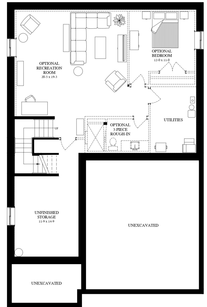
BASEMENT 1195 Sq. Ft. Optional Finished Basement
