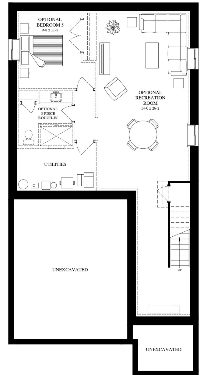
BASEMENT 1024 Sq. Ft. Optional Finished Basement
