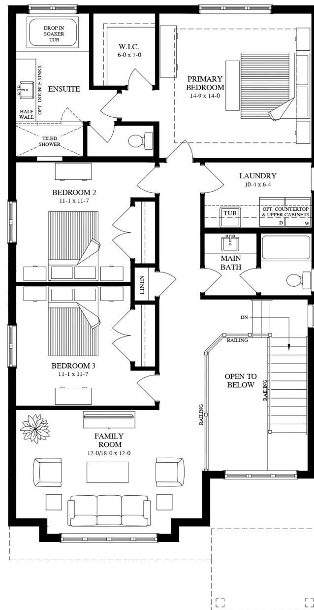
SECOND FLOOR 1388 Sq. Ft.
