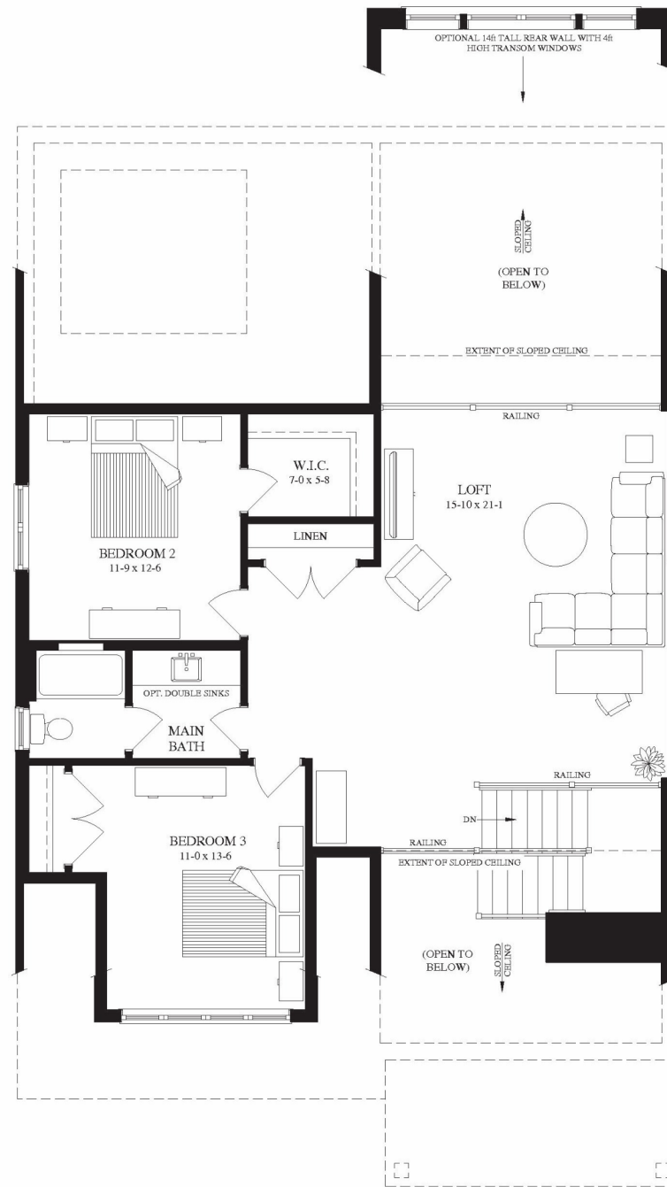
SECOND FLOOR 1063 Sq. Ft.
