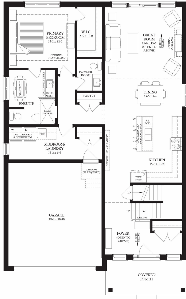
MAIN FLOOR 1505 Sq. Ft.
