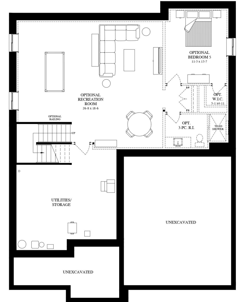
BASEMENT 1142 Sq. Ft. Optional Finished Basement
