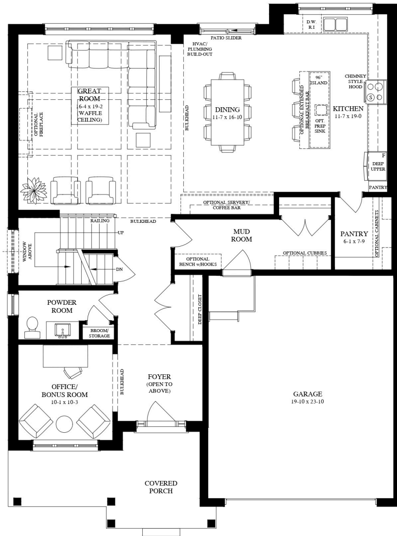
MAIN FLOOR 1522 Sq. Ft.
