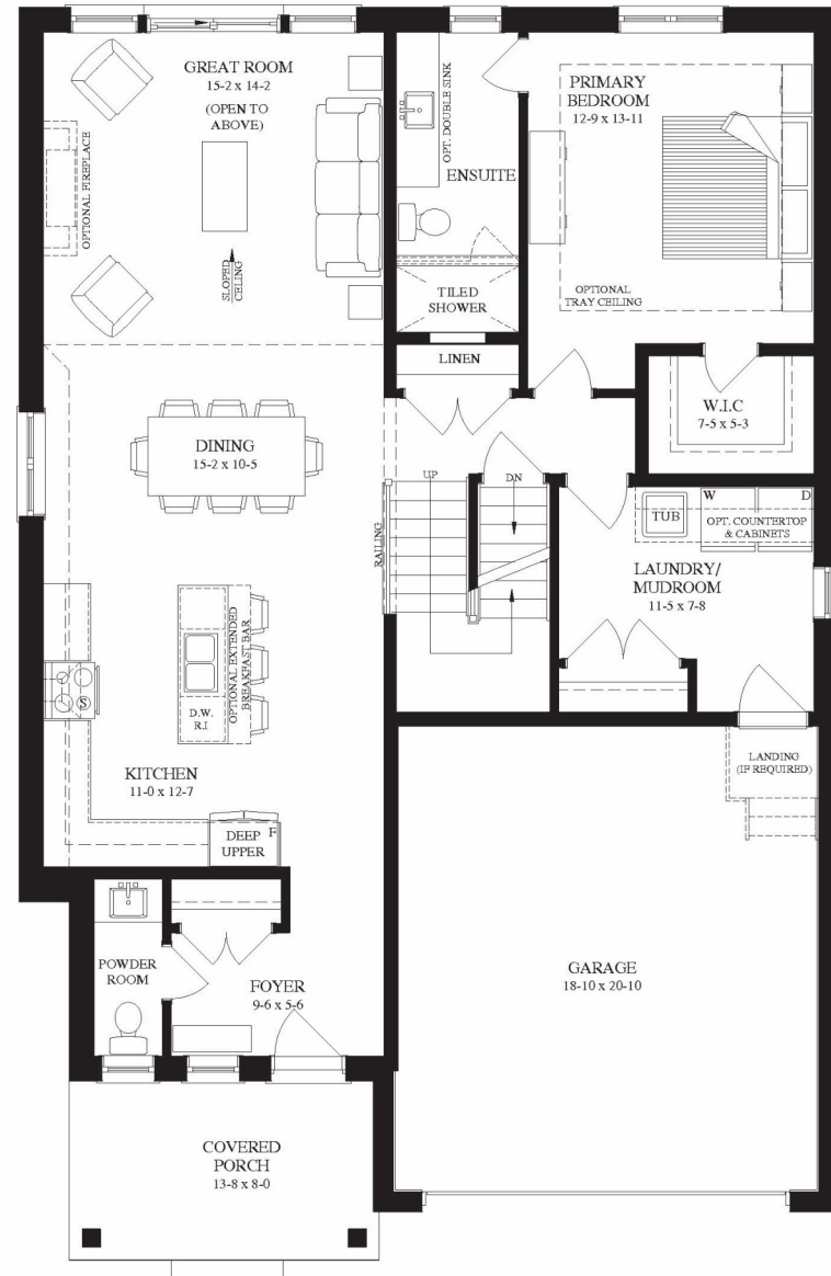
MAIN FLOOR 1402 Sq. Ft.
