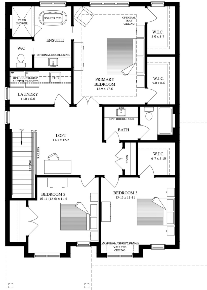
SECOND FLOOR 1363 Sq. Ft.
