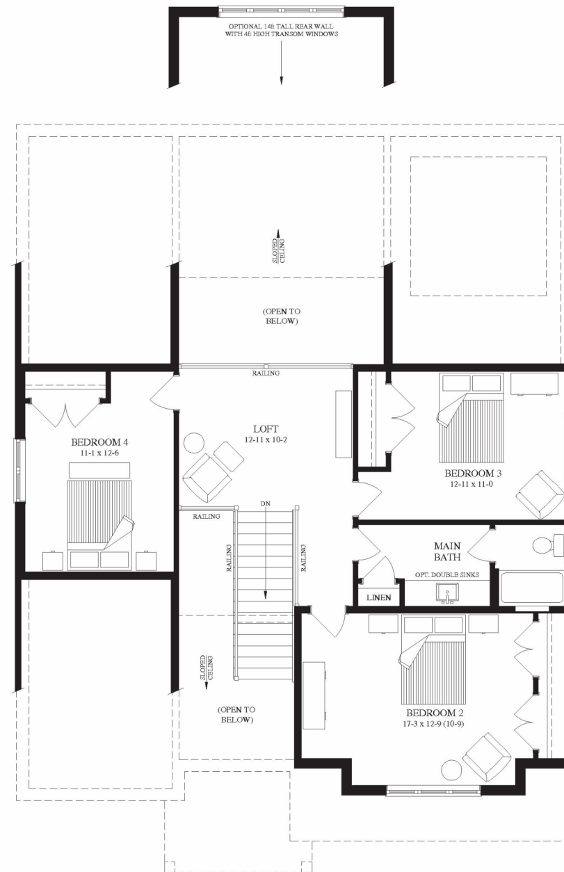
SECOND FLOOR 993 Sq. Ft.
