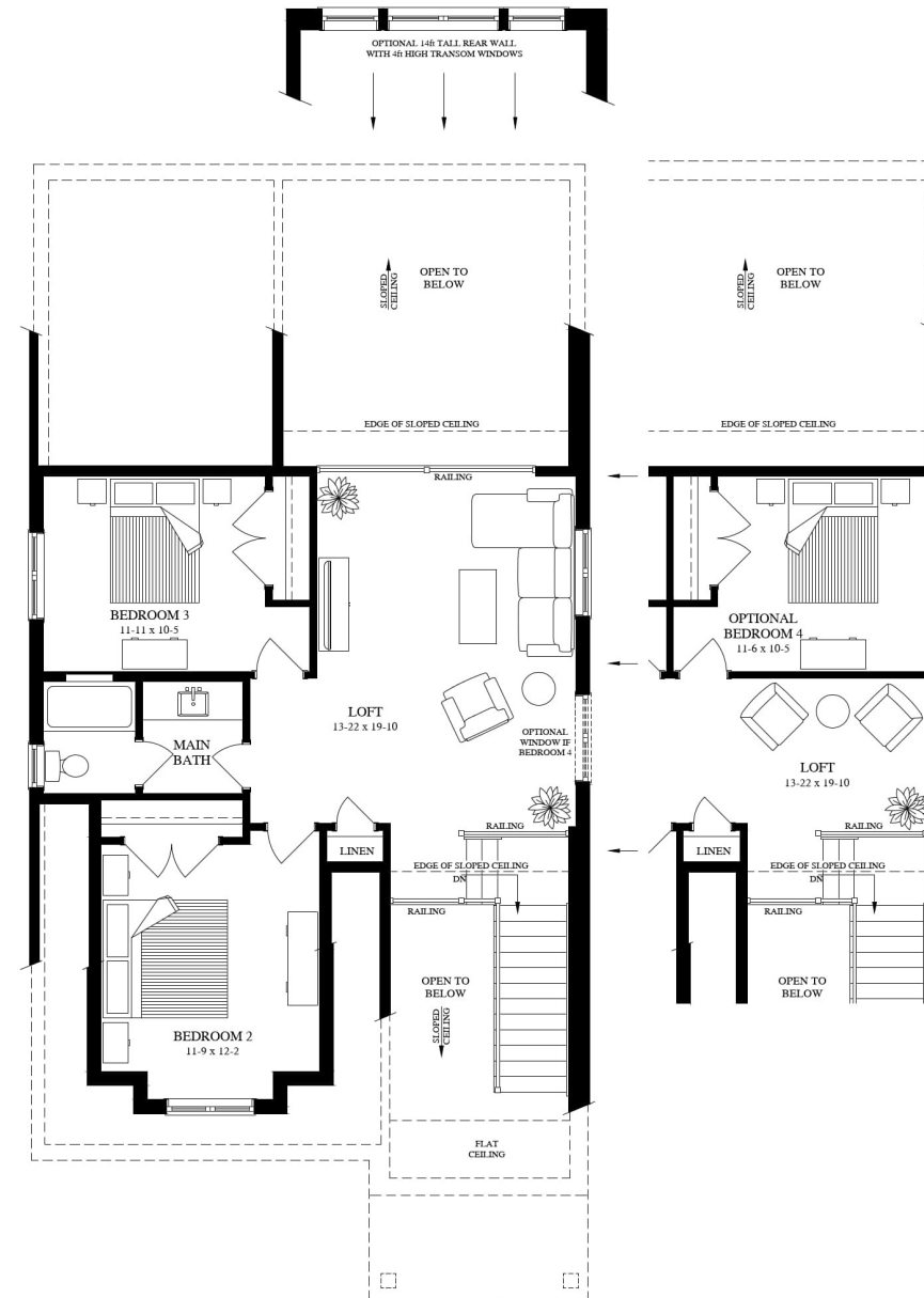
SECOND FLOOR 860 Sq. Ft.
