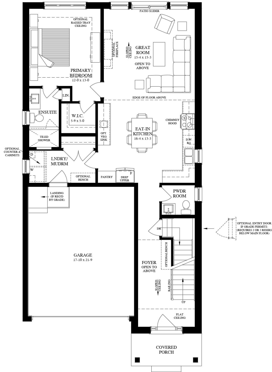
MAIN FLOOR 1195 Sq. Ft.
