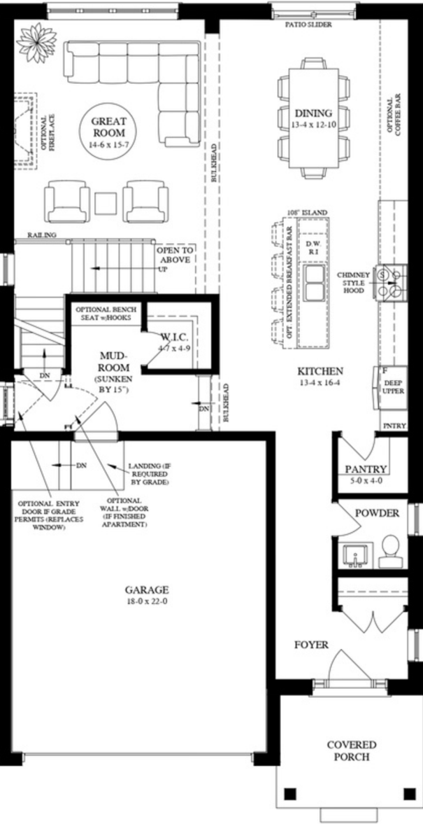
MAIN FLOOR 1114 Sq. Ft.
