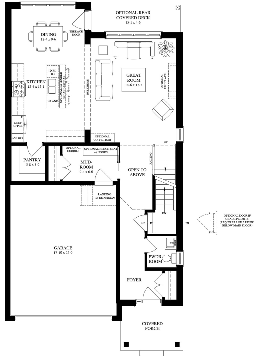
MAIN FLOOR 1065 Sq. Ft.
