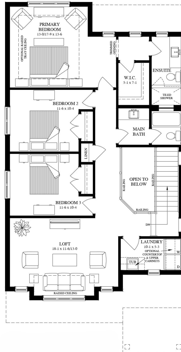
SECOND FLOOR 1345 Sq. Ft.
