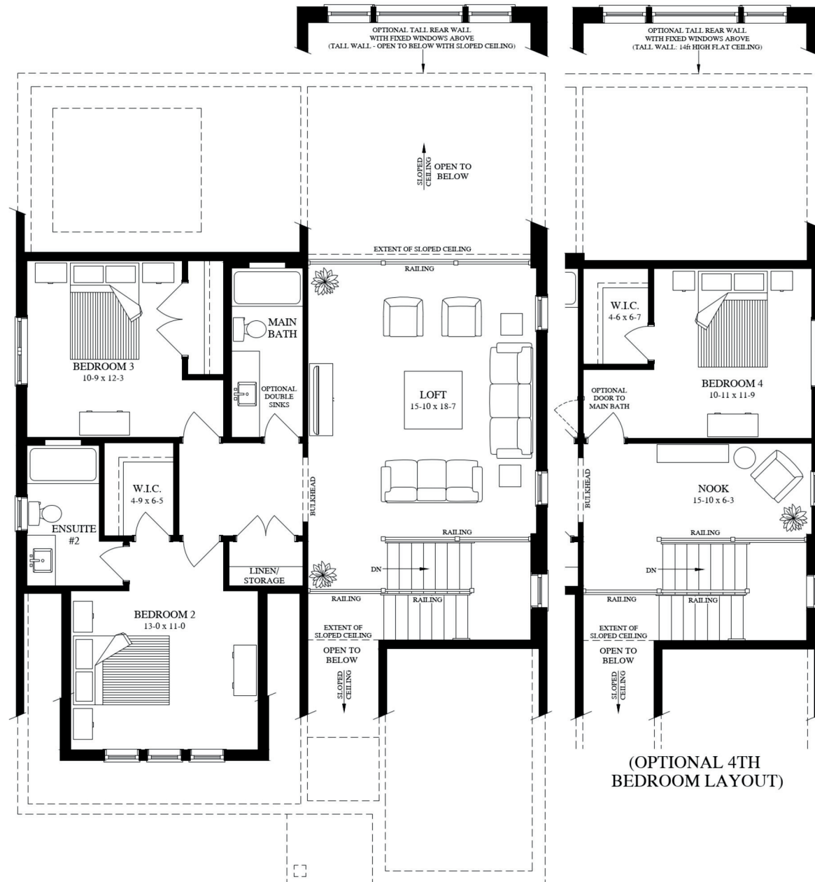
SECOND FLOOR 1063 Sq. Ft.
