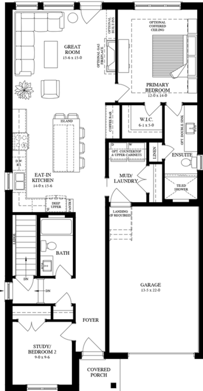
MAIN FLOOR- LAYOUT 1 1323 Sq. Ft.
