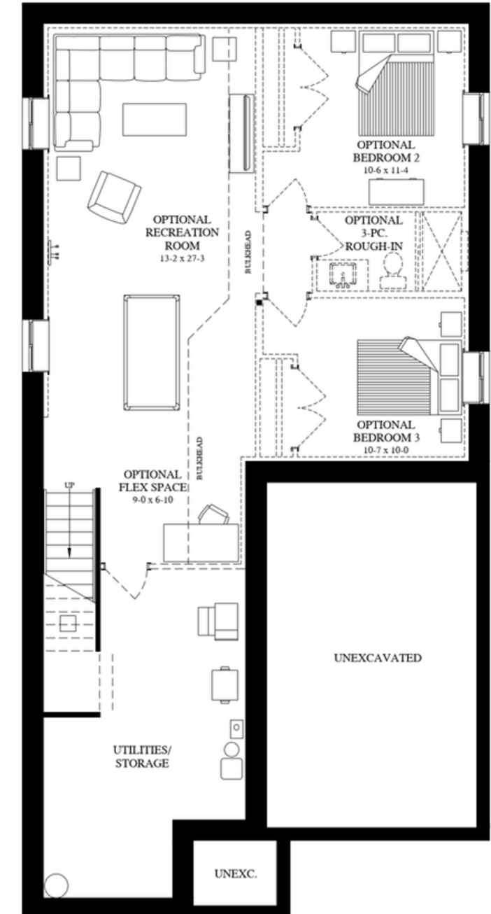
BASEMENT 1024 Sq. Ft. Optional Finished Basement
