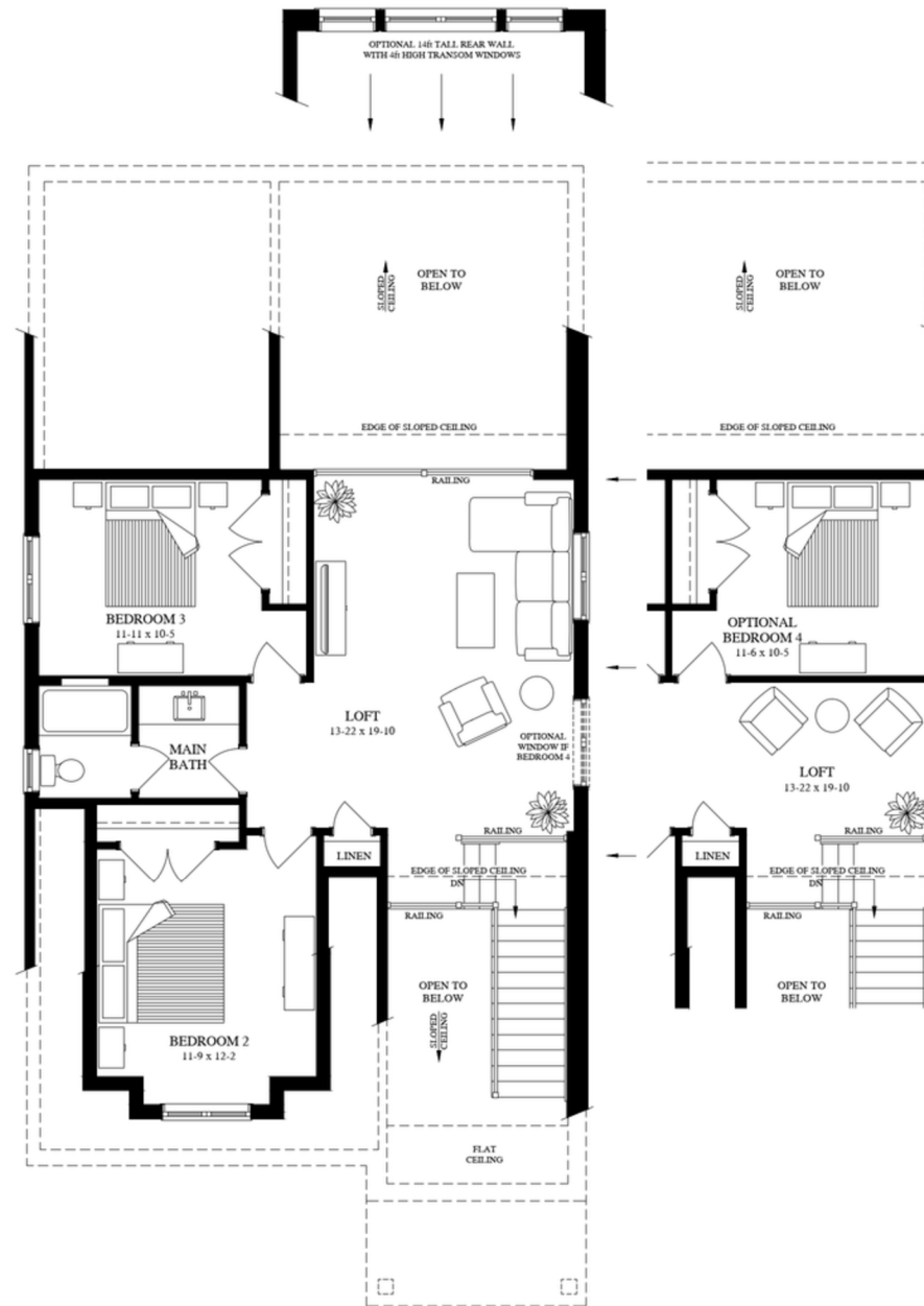
SECOND FLOOR 860 Sq. Ft.
